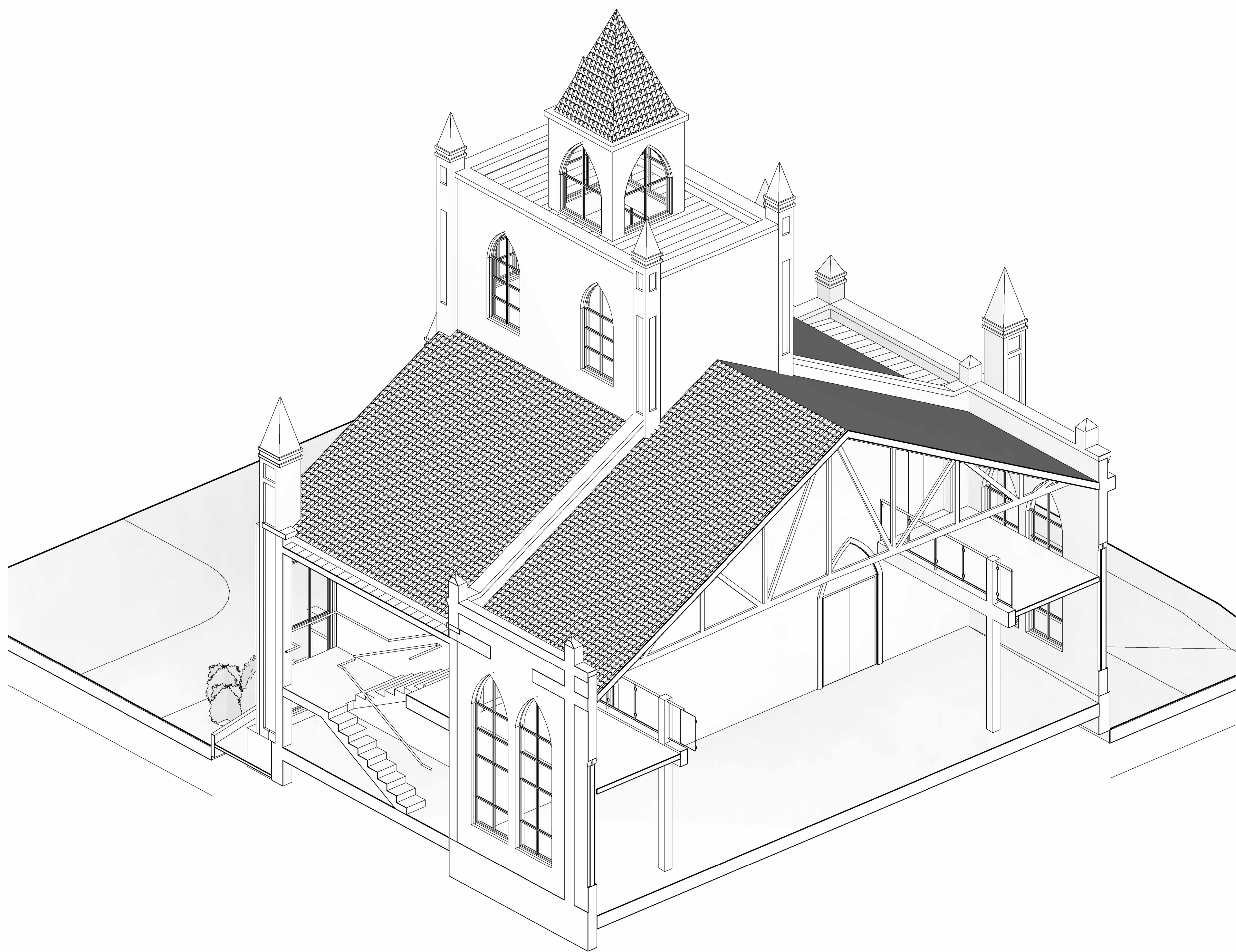
1 3D_ShortSection
